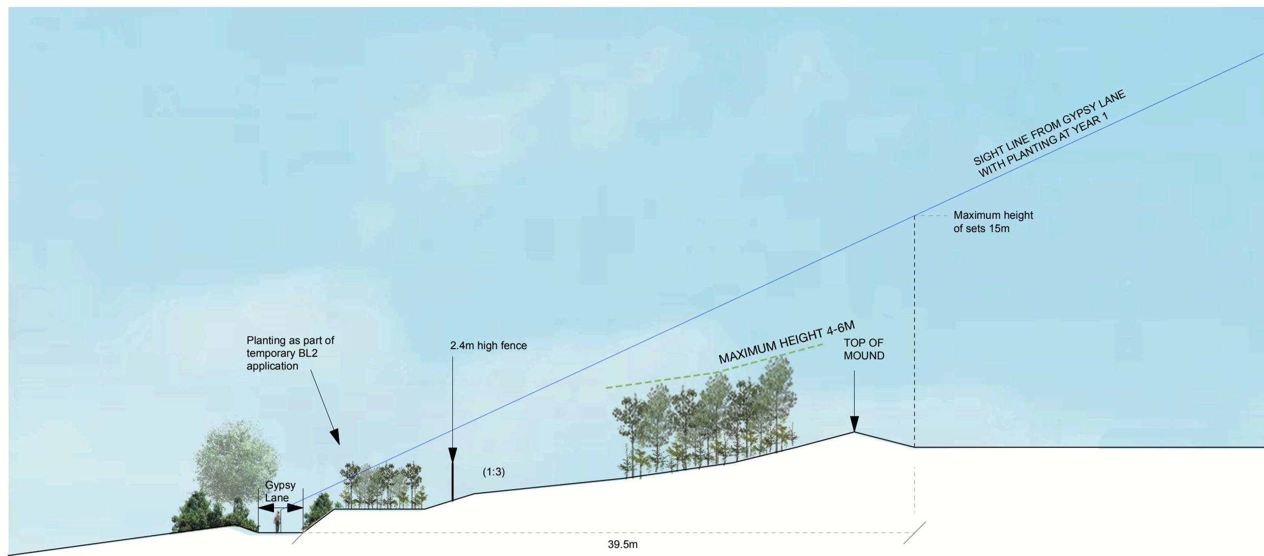
Section A-A - Year 1
